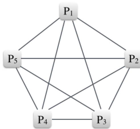
Figure 1.5: Complete Network of Size 5, K_5
