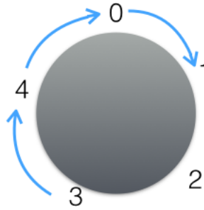
Figure 2.5: Clock-Wise Order of i . i = 3 in: 324 \rightarrow 241 .
