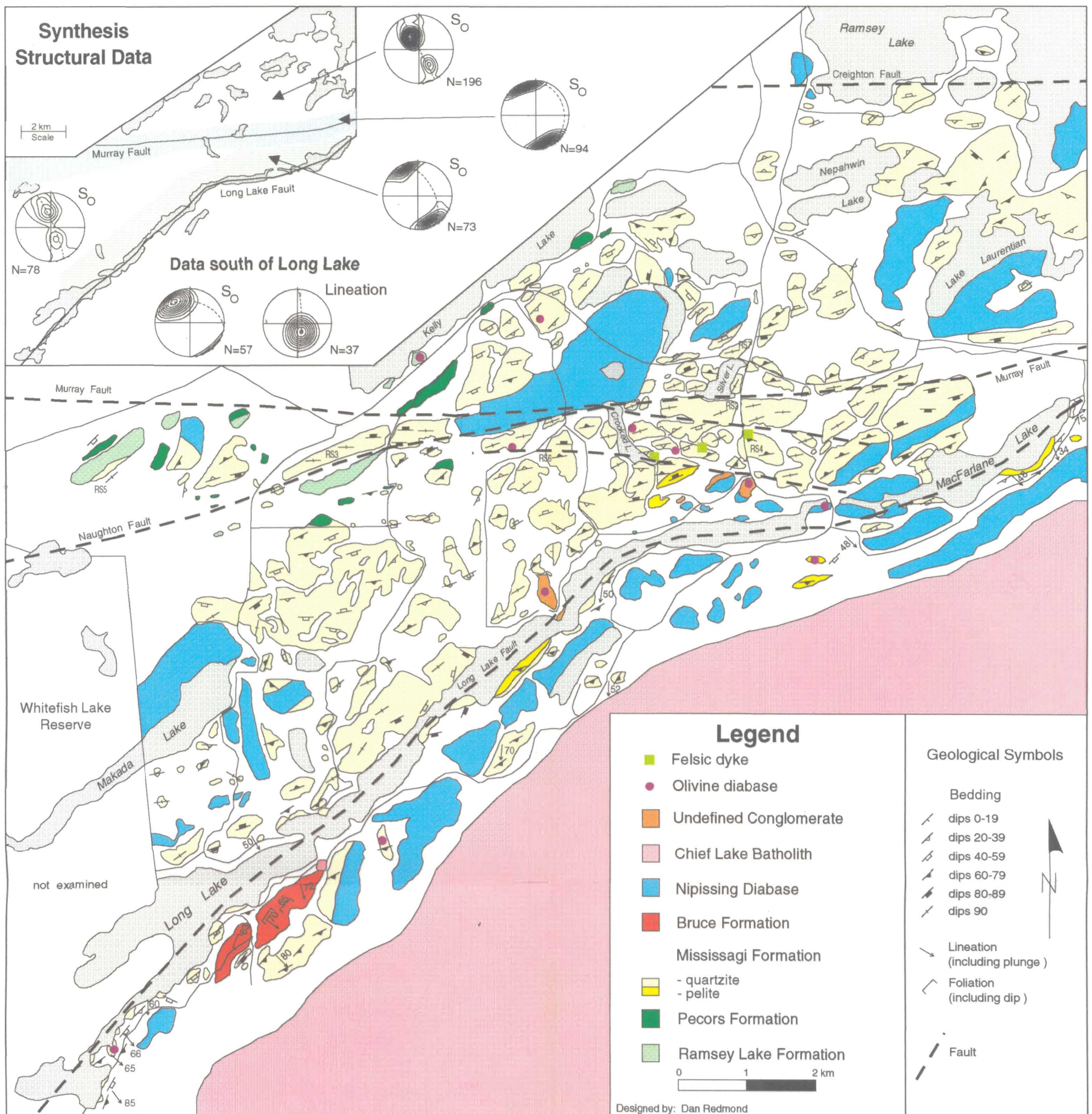
Figure 4.1: Geological map of the study area. Insert in the top left displays plots of bedding poles and lineations from different sections of the study area.
